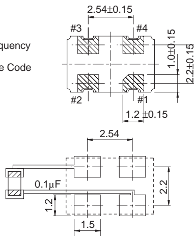
Recommended soldering pattern
